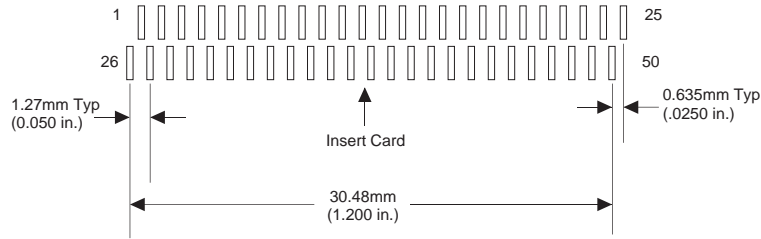
Figure 8 Two Row SMT Host PCB Pattern
