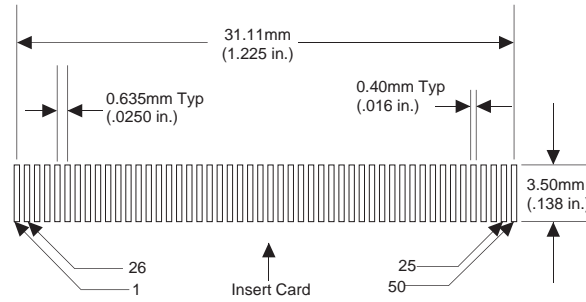
Figure 9 Single Row SMT Host PCB Pattern
