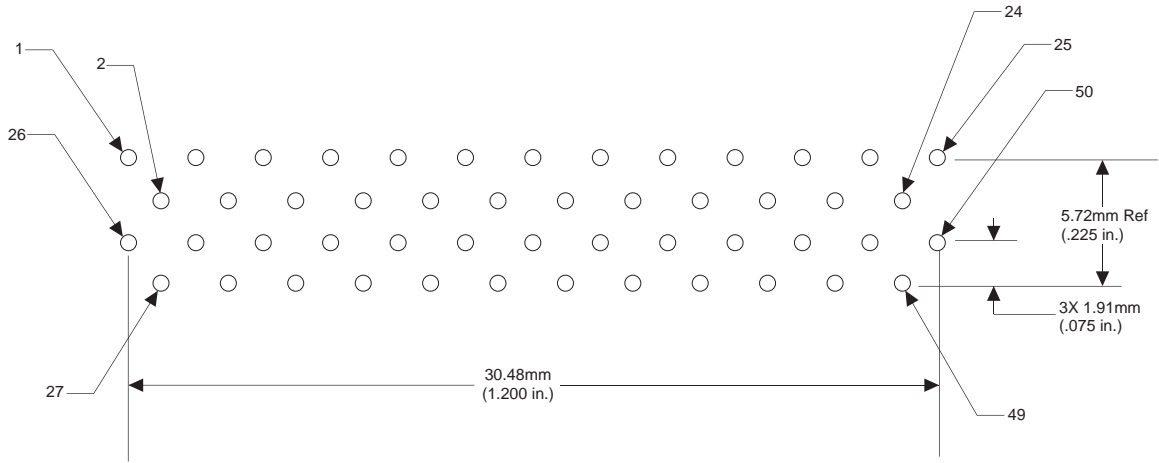
Figure 11 Vertical Through Hole Host PCB Pattern
