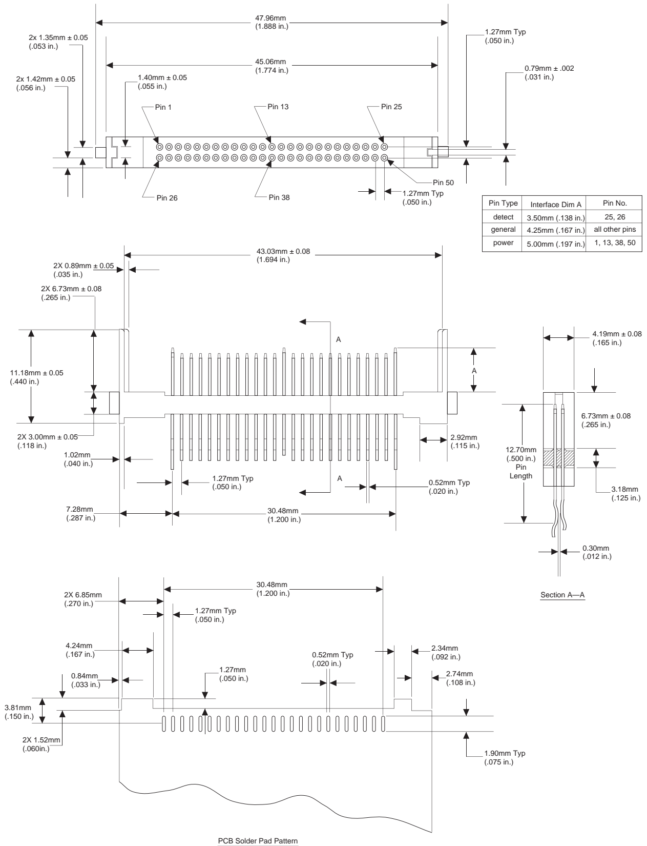
Figure 6 Straddle Mount CF Card Adapter Header
