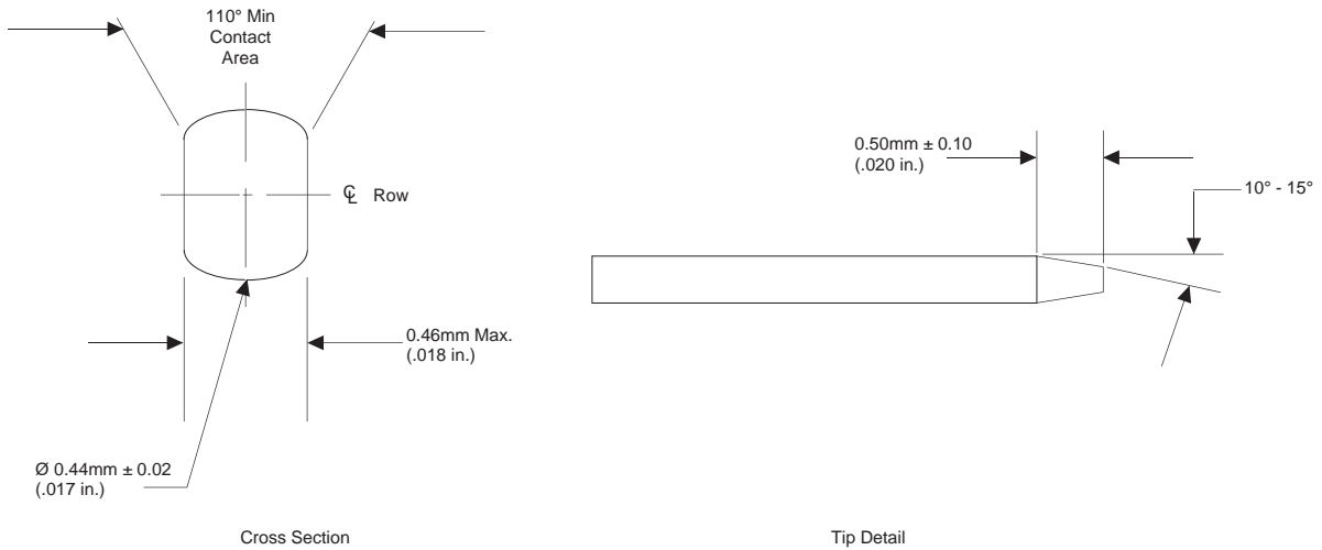
Figure 5 Header Pin Detail
