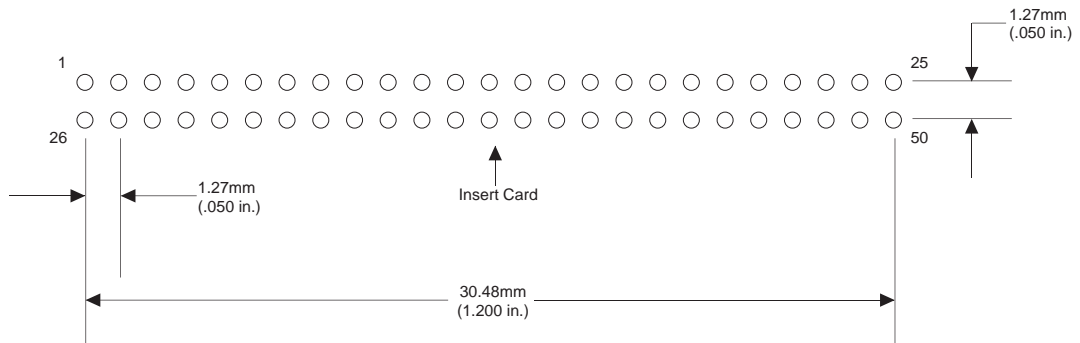
Figure 12 Alternate Right Angle Through Hole Host PCB Pattern
