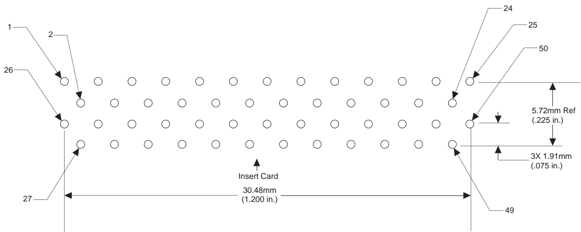
Figure 10 Right Angle Through Hole Host PCB Pattern
