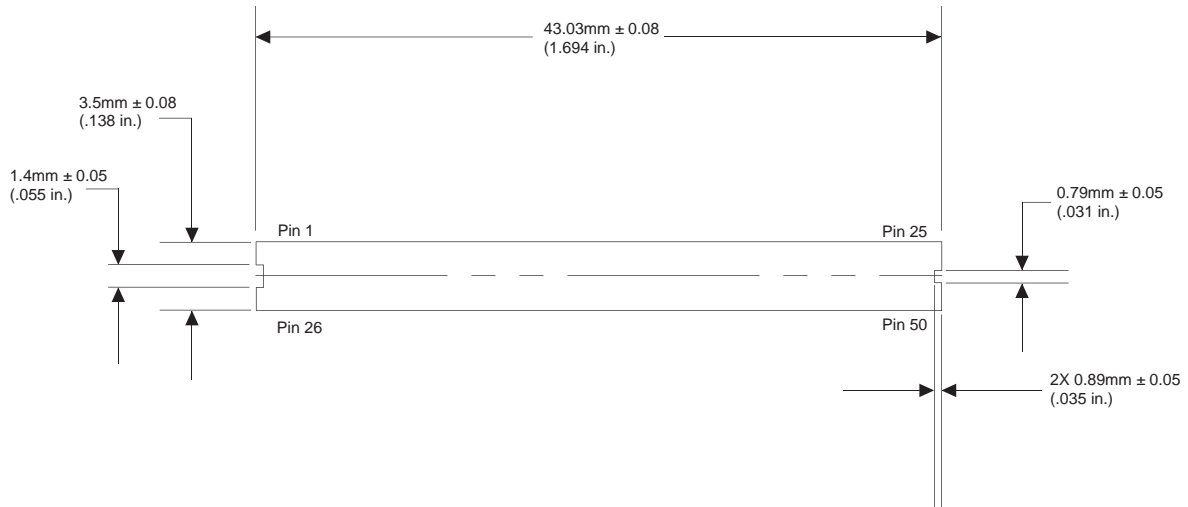
Figure 4 Pin Connector Opening
