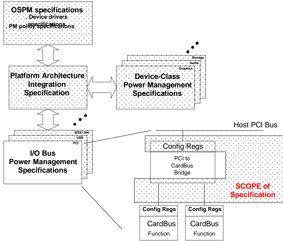
Figure 3-1: Operating System Directed Power Management System Architecture
