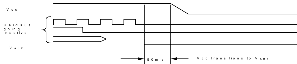
Figure 3-10: V_{CC} to V_{AUX} Transitioning
