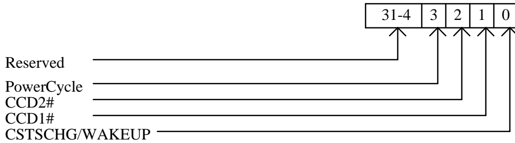
Figure 4-1: Event Register
