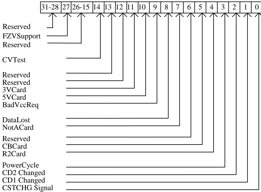
Figure 4-4: Force Register
