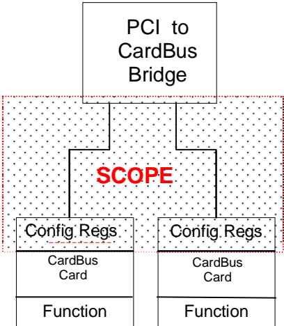
Figure 3-7: Non-Bridge CardBus Function Power Management Diagram
